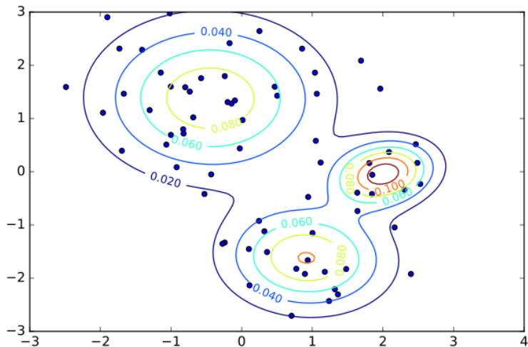
Mixture of Gaussian model.
