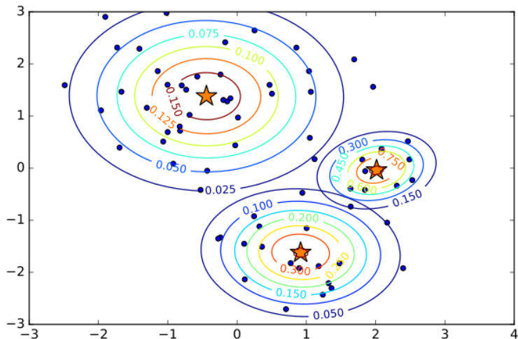
Individual Gaussians in the model.
