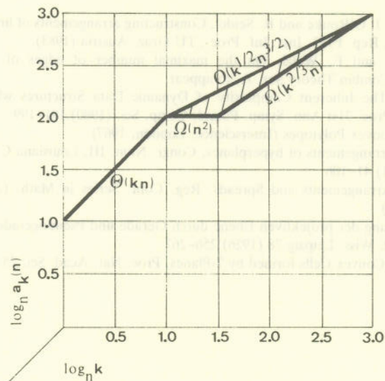
Fig. 3. Asymptotic results on a_k(n) .
