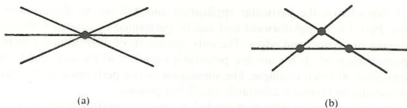
Fig. 2. Perturbing a non-simple arrangement. (a) Degenerate case. (b) Perturbed arrangement.
