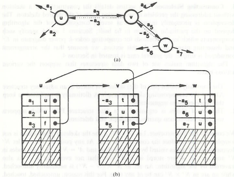
Fig. 1. Representing a skeleton graph. (a) Incomplete skeleton graph. (b) Adjacency lists.
