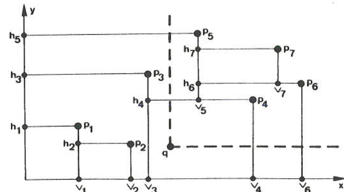
Fig. 1. The map for (p_1, p_2, \dots, p_7) and query point q .
