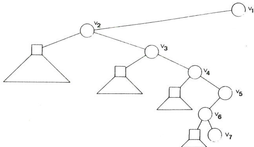
Fig. 5. Set V = (v_1, v_2, \dots, v_7) and nodes in W .
