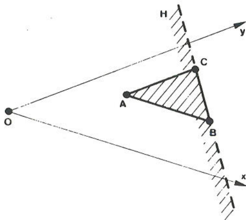
Fig. 4. Range query with triangle ABC .
