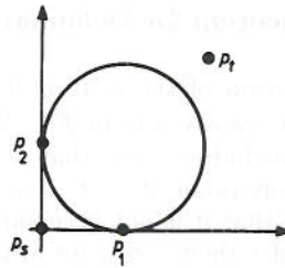
Fig. 3. Points p_s and p_t are chosen so that p_1 and p_2 define an edge of the Delaunay triangulation
