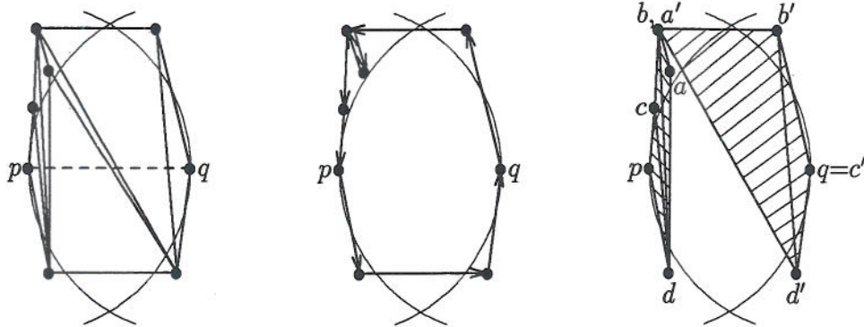
FIG. 1. To the left are the triangles of t(S) that intersect pq . If we remove the edges that intersect pq we get a polygon whose boundary is oriented in a counterclockwise order. The prefix P and the suffix Q defined for this configuration are illustrated to the right. Although b and a' are the same point, they refer to different angles of this point.
