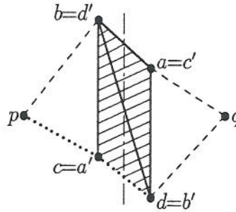
FIG. 4. If bd and b'd' are both nonswitchable, then b and d are the only convex angles besides p and q .
