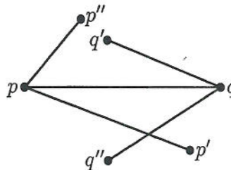
FIG. 11. By the choice of p' the counterclockwise angle \angle p'pq contains no 1-edge with pq on its beneath side. Symmetric statements hold for p'', q' , and q'' .
