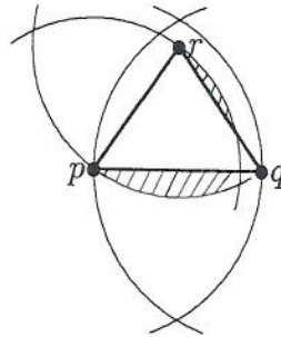
FIG. 9. Points z lie in the interior of \eta_{rp} - pqr , which consists of one or two connected components, depending on whether or not the angle at r in triangle pqr is nonacute.
