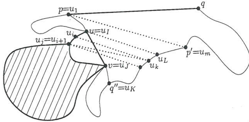
FIG. 13. The shaded portion of the pocket Y_{uv} represents the part of the triangulation t_{uu_L} beyond uu_L that is retained for the final triangulation. The remaining portion is triangulated by fanning out from v .
