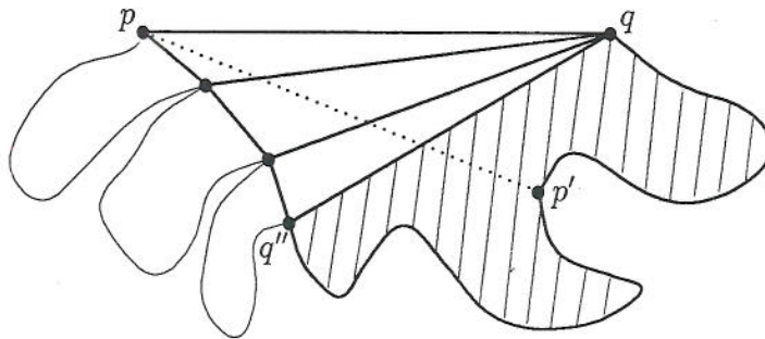
FIG. 12. The shaded portion represents the triangulation beyond qq'' ; it forms part of the final triangulation.
