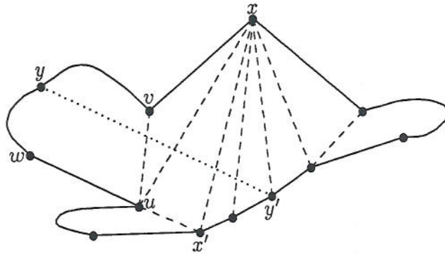
FIG. 8. Polygonal region X is triangulated by fanning out from x , connecting adjacent neighbors of x , and recursing in the thus created pockets. The illustration of this process is schematic and ignores some of the inherent shape constraints for X .
