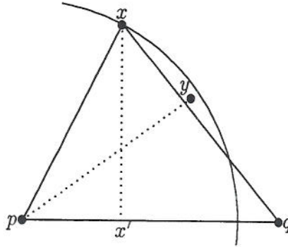
FIG. 7. Vertex x is visible from p and from q , so pqx is empty. It follows that if y \in \eta_{x\bar{p}} \cap \eta_{p\bar{q}} then pqyx is a convex quadrilateral.
