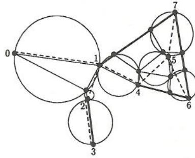
Fig. 4.1. The original graph, \mathcal{G} , has vertices 0–7 and edges 17, 23, 46, and 67. The edges of the minimum spanning tree, 01, 12, 23, 14, 45, 56, and 57, are indicated by broken lines. Each edge of the tree corresponds to a blocking circle. Each blocking circle encloses protected edges of \mathcal{H} .
