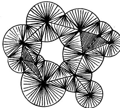
Fig. 3.1. The covering of \cup B using joins between simplices of \mathcal{K} and faces of \cup B .
