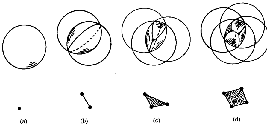
Fig. 6.1. The intersection of one, two, three, and four 3-balls. The face structure is dual to that of a vertex, an edge, a triangle, and a tetrahedron.
