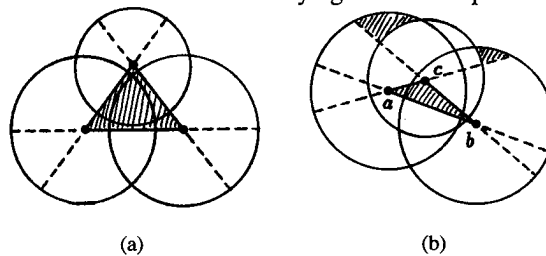
Fig. 7.2. The three disks to the left define a favorable case, whereas the disks to the right do not. Indeed, the intersection of the disk around b with the half-plane opposite ac is not covered by the disks around a and c . The same is true for the disk around a and the half-plane opposite bc .
