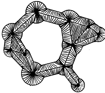
Fig. 3.2. This is \Phi(\cup B, \frac{1}{2}) : at time t = \frac{1}{2} the fringe is narrowed to half the original width.
