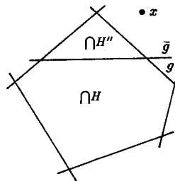
Fig. 5.2. \cap H' is the union of \cap H and \cap H'' . Since x \notin \cap H , by assumption, we have x \in \cap H' iff x \in \cap H'' .
