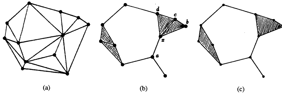
Fig. 2.3. The diagrams \mathcal{D} , \mathcal{N} , and \mathcal{S} of the 12 disks in Fig. 2.1 are shown from left to right. By the definition of nerve, \mathcal{D} is dual to the Voronoi diagram in Figure 2.2(a) and \mathcal{N} is dual to the decomposition of the union defined by \mathcal{L} .
