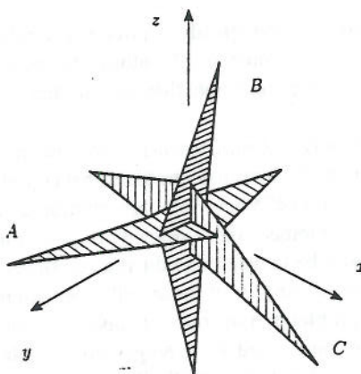
Fig. 4. All three groups A , B , and C together—the full counterexample.
