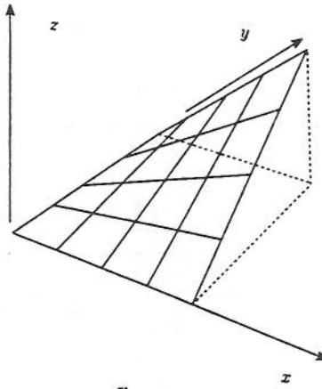
Fig. 1. The hyperbolic paraboloid z = xy and its two families of generating lines.
