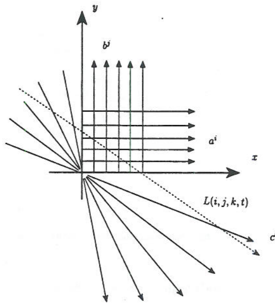
Fig. 2. The oriented line groups A, B, C (solid) and a representative of the oriented lines L(i, j, k, t) (dashed), viewed from above.
