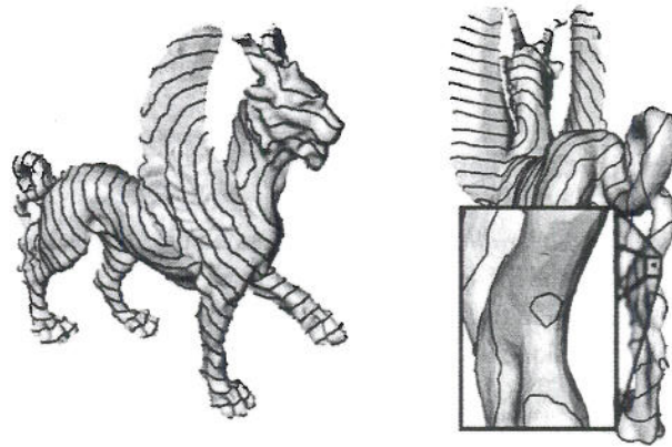
Fig. 19. Simulation of the wave-front propagation in [103].
