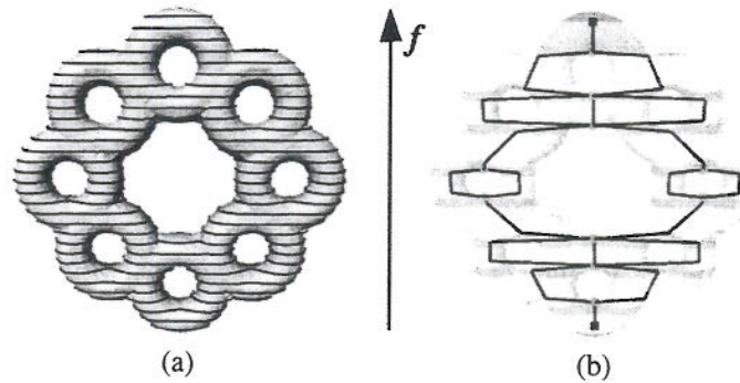
Fig. 21. A surface, (a), and its Reeb graph representation with respect to the height function, (b).
