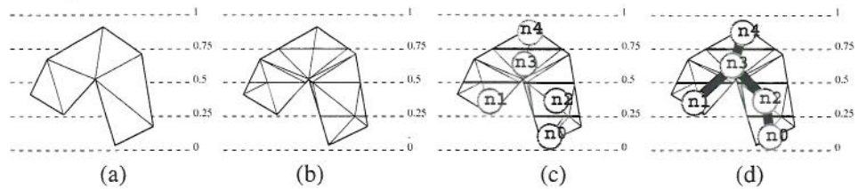
Fig. 22. Pipeline of the Reeb graph extraction in [73]. (b)
