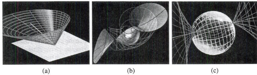
Fig. 5. The bisector sheets (in red/magenta) of a plane and a line (a), a sphere and a canal surface (b), and a line and a sphere (c).
