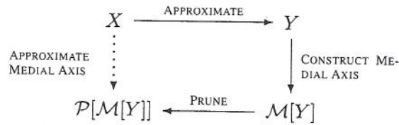
Fig. 7. An approximation \mathcal{P}[\mathcal{M}[Y]] of the medial axis of a shape X can be found as part of the medial axis of a shape Y approximating X .
