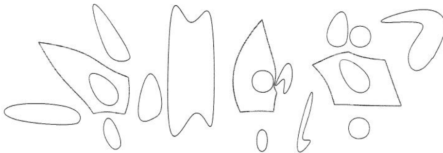
Fig. 6. Three examples of precise Voronoi regions (in gray wide lines) of rational closed parametric curves. The Voronoi region of one curve (the curve inside the Voronoi region) is shown in each example.
