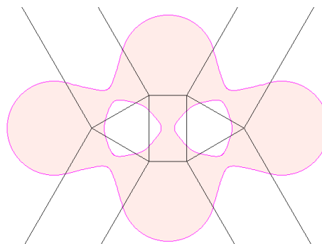
FIGURE 68.3.2 The skin curve defined by four circles in the plane. The mixed complex decomposes the curve into pieces of circles and hyperbolas.
