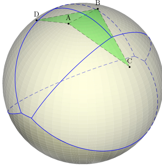
■ Figure 2 The Voronoi domains of four points on the 2-dimensional sphere. The darker region in the south does not belong to any of these domains because the four points all belong to the northern hemisphere. The dual Delaunay complex consists of two triangles glued along a shared edge.
