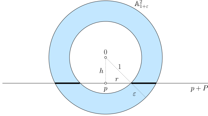
■ Figure 3 For h = \|p\| < 1 , the slice of the (n+1) -dimensional annulus is a k -dimensional annulus. In this picture, n+1 = 2 and k = 1 .
