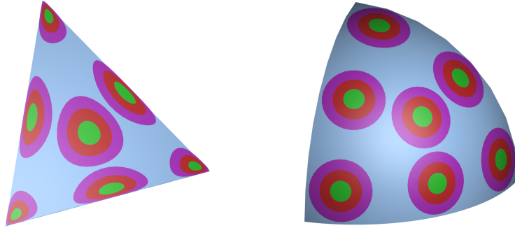
■ Figure 1 Left : disk neighborhoods under the Fisher information metric of seven points in the standard triangle. Right : the corresponding seven points and cap neighborhoods in the isometric non-negative octant of the 2-sphere. For aesthetic reasons, the octant is scaled to 1/\sqrt{2} times its actual size.
